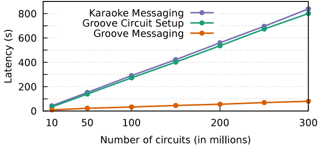
Figure 7: Latency of circuit setup and messaging rounds with respect to the number of circuits. The figure also compares with Karaoke’s messaging round as a baseline (1 user relationship in Karaoke equals 2 Groove circuits) [19]. The mixnet has 100 servers.
